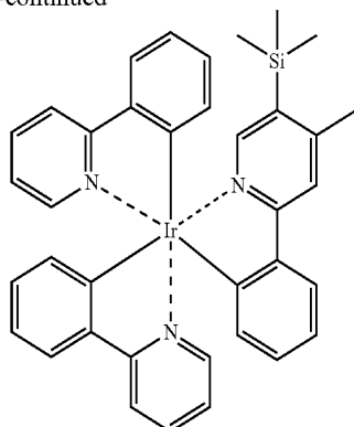
Comparative Compound 1
