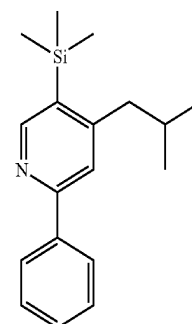
Compound A1
