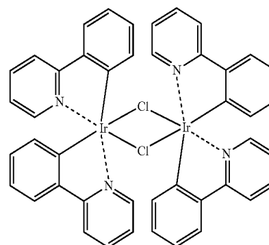
Compound M2A
