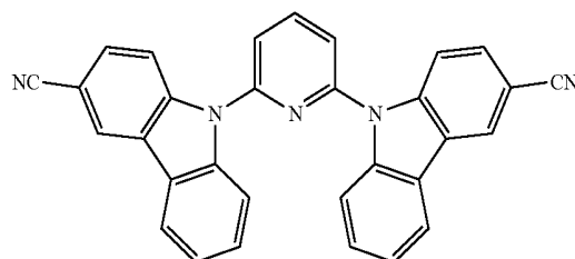
Compound H51
