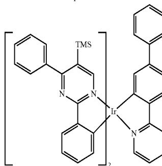
Compound A'
