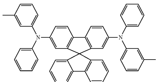
Spiro-TPD
